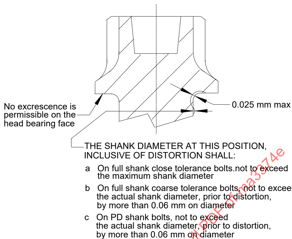
Figure 1 - Permissible distortion from fillet working
