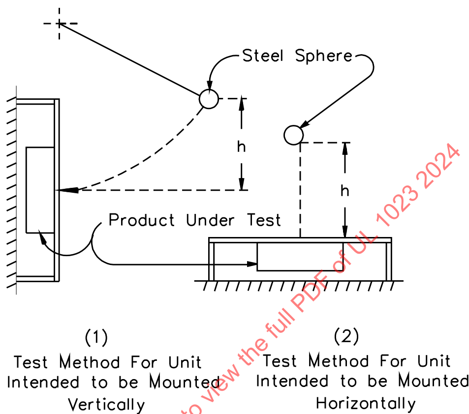
Figure 41A.1 Jarring Test
