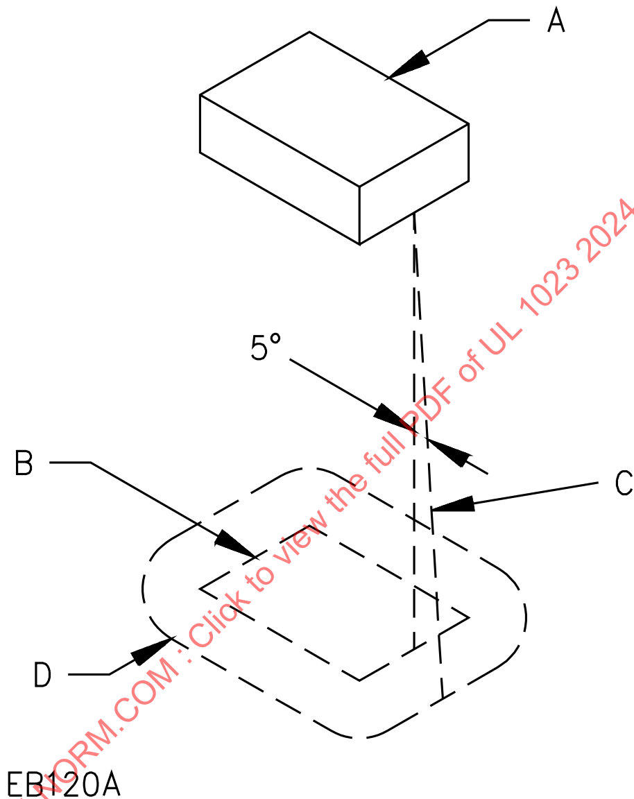
Figure 10.1 Protective pan
