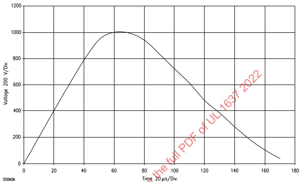
Figure 48.2 Signal line transients – 1000V curve
