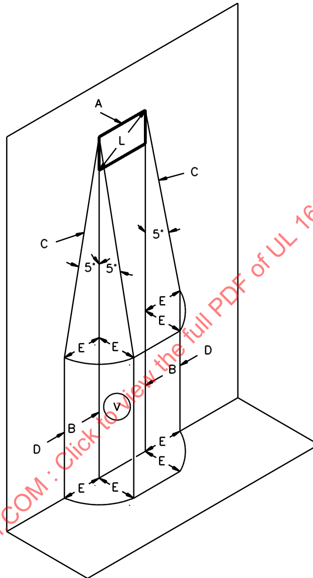
Figure 8.3 Example of enclosure side opening
