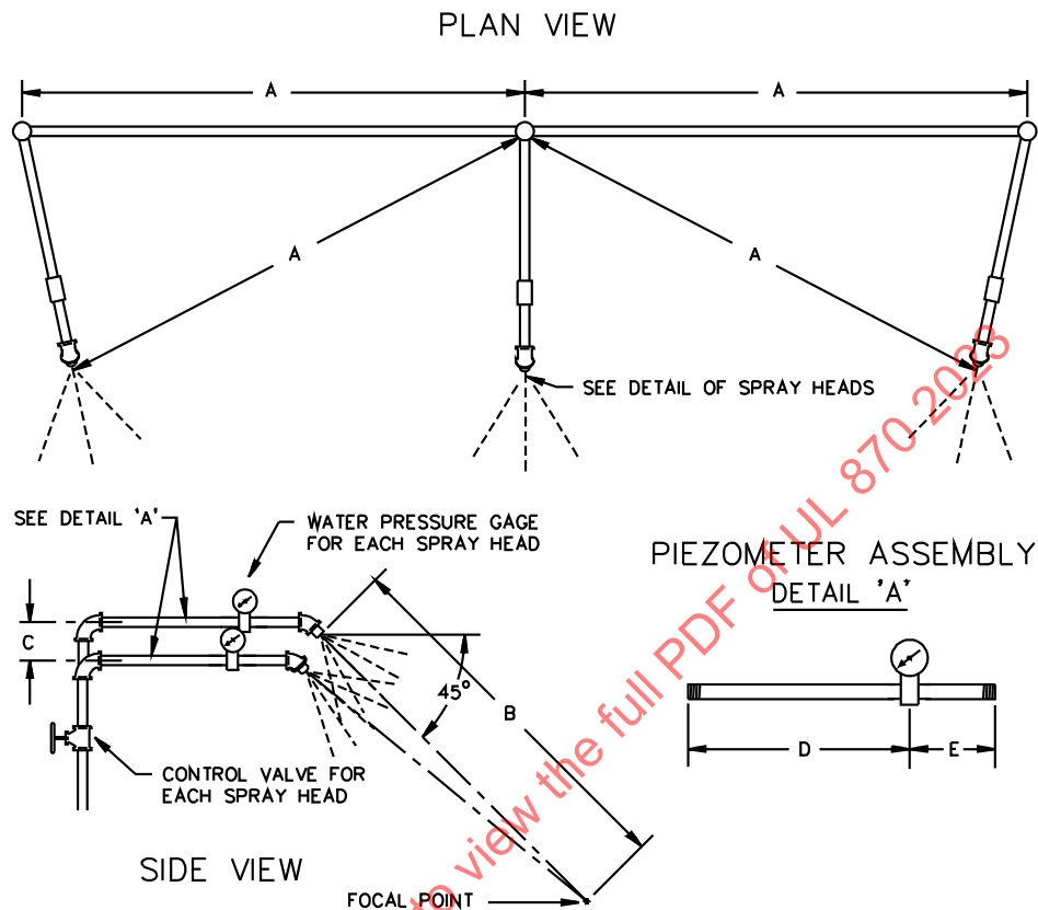
Figure 20.1 Rain-test spray-head piping
